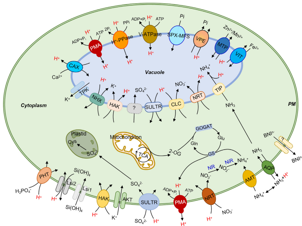
Figure 2. Roles of plasma membrane \text{H}^+ -ATPases (PMAs) in the uptake and/or assimilation of mineral nutrients by providing proton motive force or membrane potential for various nutrient transporters. Abbreviations: AKT, arabidopsis \text{K}^+ transporter; AMT, ammonium transporter; AOA, ammonia-oxidizing archaea; AOB, ammonia-oxidizing bacteria; AQP, aquaporin; BNI, biological nitrification inhibitor; CLC, chloride channel; Gln, glutamine; Glu, glutamate; GOGAT, glutamate synthase; GS, glutamine synthetase; HAK, high-affinity potassium transporter; Lsi, Low silicon; MTP, metal tolerance protein; NHX, \text{Na}^+/\text{H}^+ antiporter; NiR, nitrite reductase; NR, nitrate reductase; NRT, nitrate transporter; 2-OG, 2-oxoglutarate; SPX-MFS, SYG1, PHO81, and XPR1 (SPX), major facilitator superfamily (MFS) protein; SULTR, sulfate transporter; TCA, tricarboxylic acid cycle; TIP, tonoplast integral protein; TPK, two-pore \text{K}^+ channel; VIT, vacuolar iron transporter; VPE, vacuolar phosphate efflux transporter.
